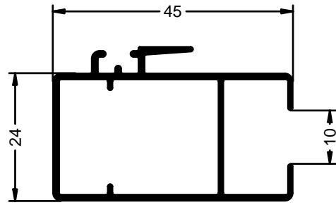
HOJA CENTRAL
