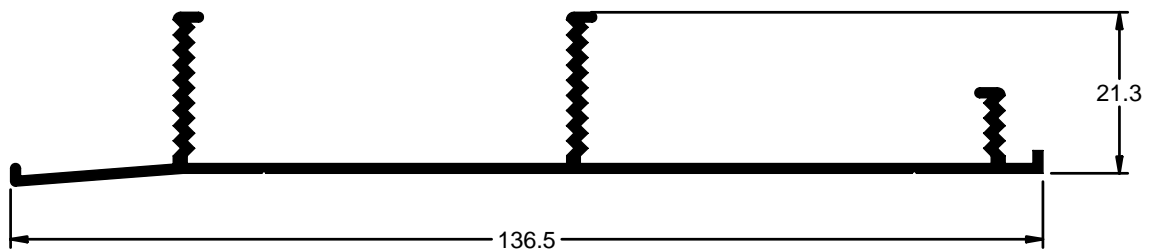
PREMARCO VERTICAL
