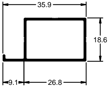
PREMARCO 36mm
