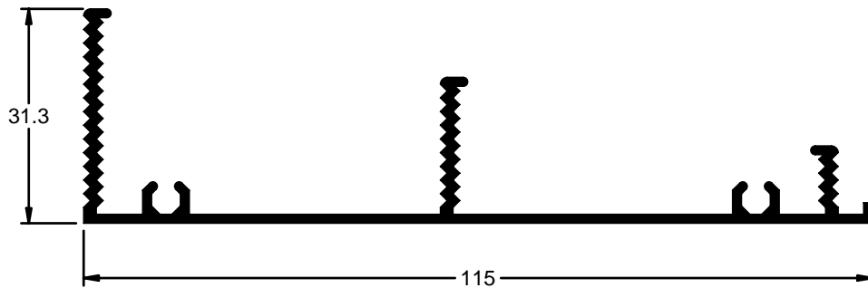
PREMARCO HORIZONTAL
